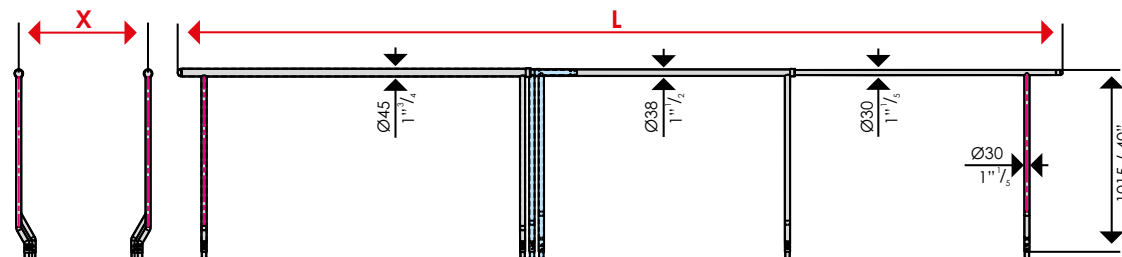
Duble side - Single handrail
