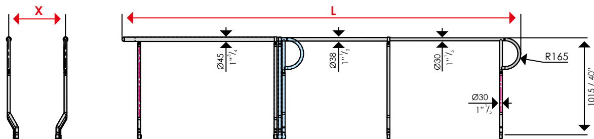
Duble side - Single handrail with handle
